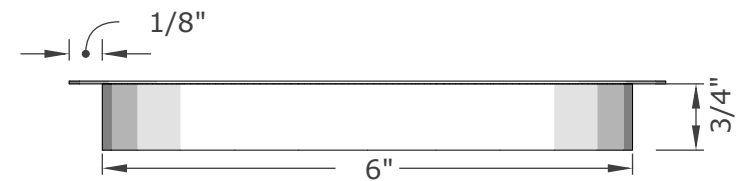
SIDE VIEW
