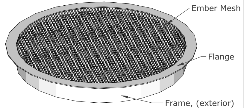
ISOMETRIC VIEW
