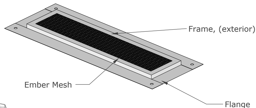
ISOMETRIC VIEW
