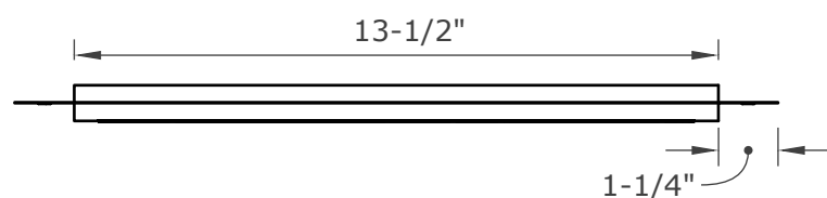
FRONT VIEW
