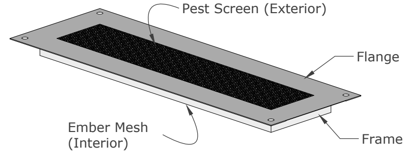
ISOMETRIC VIEW
