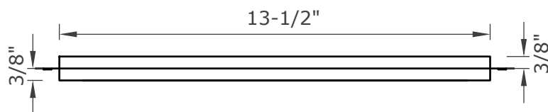
FRONT VIEW
