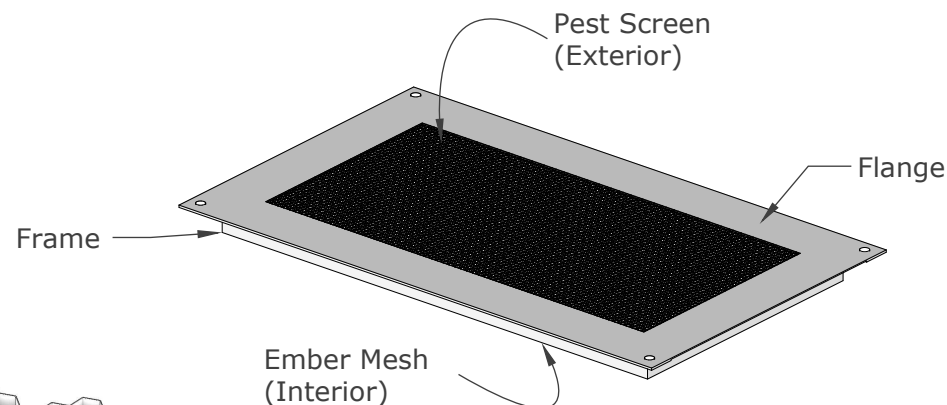
ISOMETRIC VIEW
