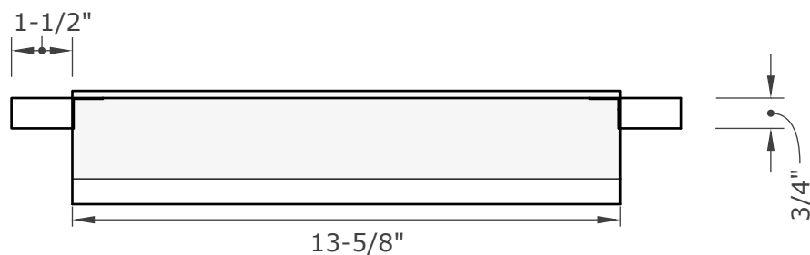
END VIEW
