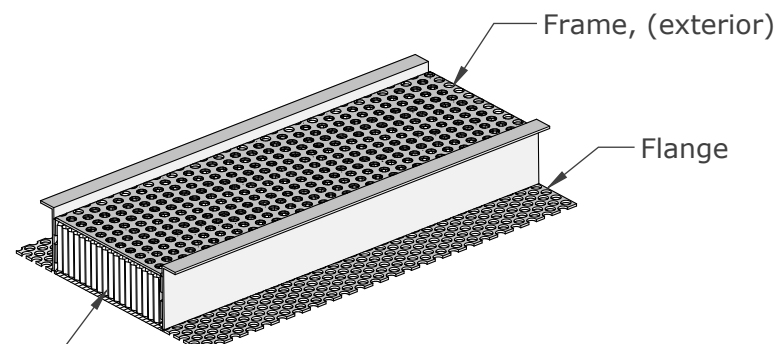
ISOMETRIC VIEWS
