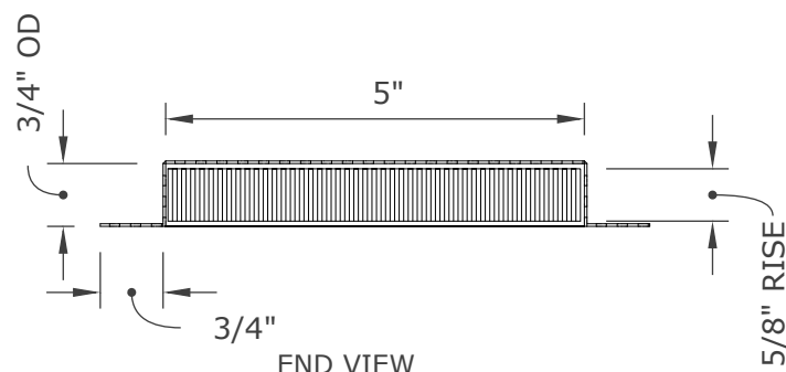
END VIEW
