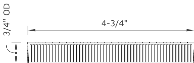
END VIEW
